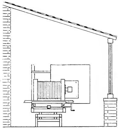
FIG. 11c.—Lean-to Side-light Studio
